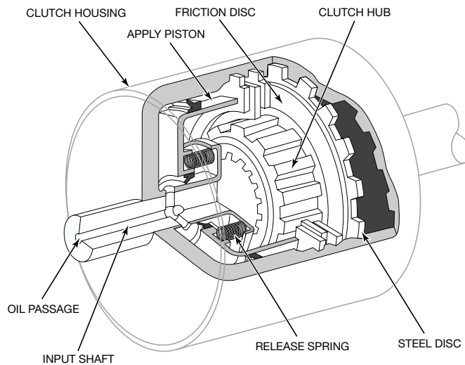
CLUTCH RELEASED
