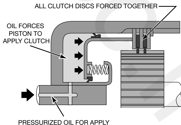
CLUTCH APPLIED
