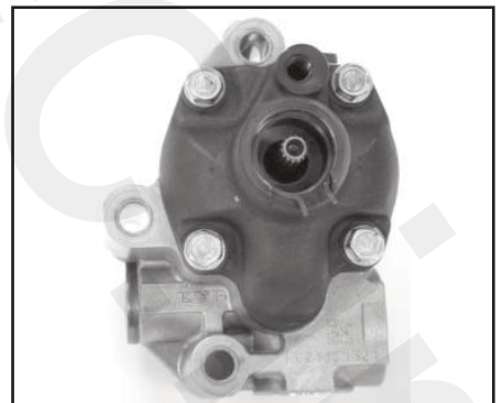
Torque cover bolts 19 Ft. Lbs. (26Nm)
