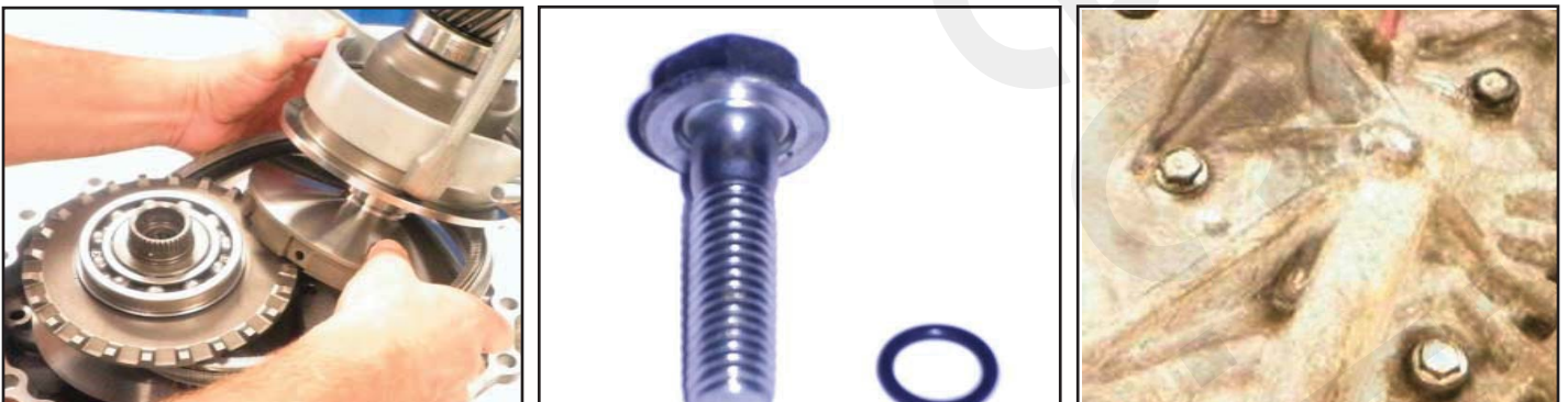
Compress secondary pulley, using new o-ring on the bolts. Torque Bolts to 33 Ft. Lbs. (45N).
