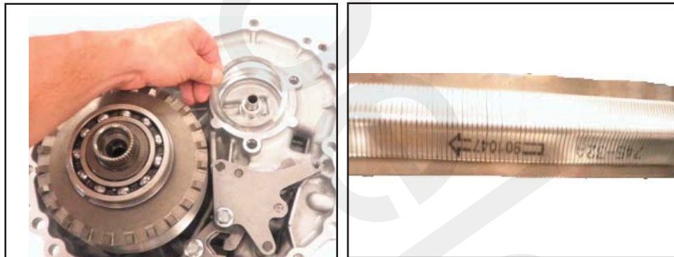
Install thrust washer for secondary pulley
