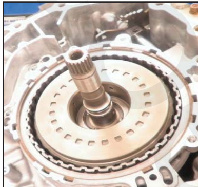
Install forward drum, drum is fully seated top of drum even with carrier
